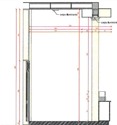
Section 0 1:20
